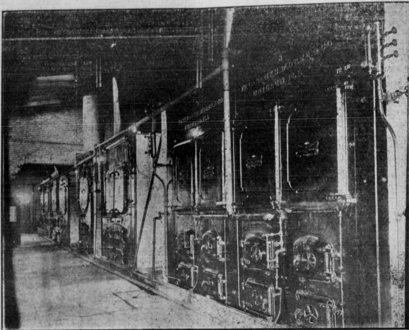
INTERIOR OF BOILER ROOM PORTLAND GENERAL ELECTRIC COMPANY STEAM PLANT, SALEM, OREGON. 800 HORSE POWER. OIL BURNERS.
