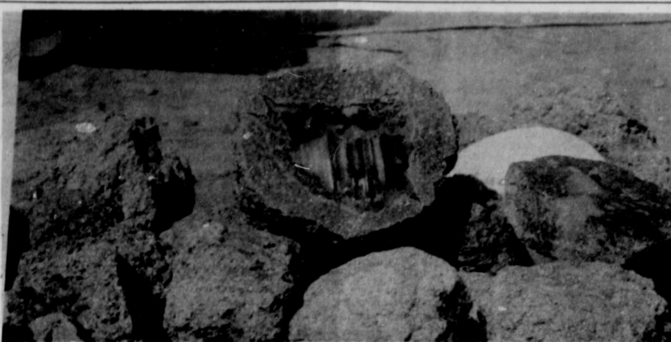
THUNDEREGGS before and after cutting.
