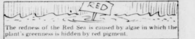
The redness of the Red Sea is caused by algae in which the plant's greenness is hidden by red pigment.
