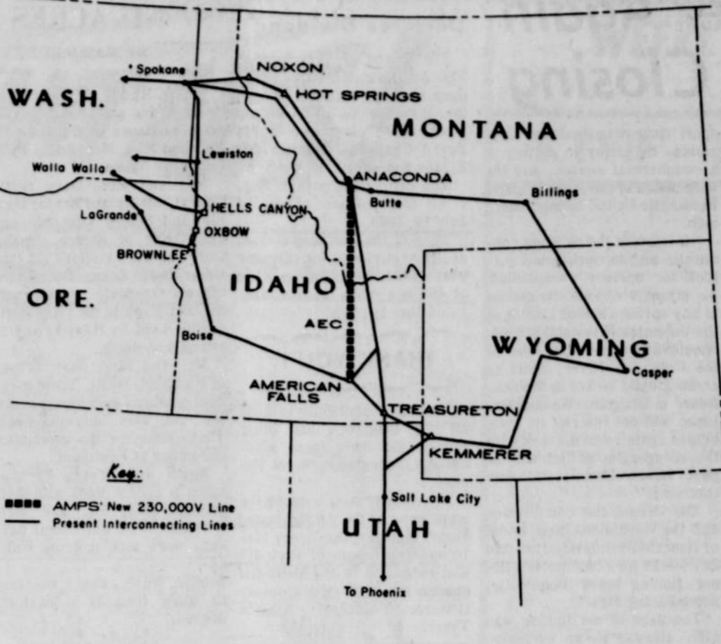
MAP SHOWS SECTION OF NEW 230,000-volt transmission line Idaho Power Company will build as one of final links in additional facility extending 565 miles between Noxon and Kemmerer to interconnect five Northwest utilities. Idaho Power plans to start work June 1 on its 60-mile section from American Falls to Scoville, near Atomic Energy Commission's testing station. Five companies will operate line as coordinating group called AMPS (Associated Mountain Power Suppliers).
