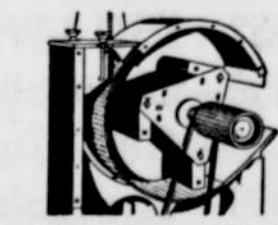
Grinding chamber of Mix-All features more hammers, larger grinding surface than any other farm mill.
