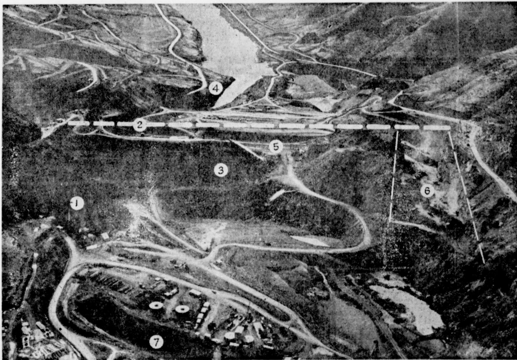
HARNESSING THE SNAKE RIVER AT BROWNLEE. 1. Powerhouse construction area. 2. Broken line shows future crest of dam 400 feet high, 1,380 feet in length. Reservoir will extend 5 1/2 miles. 3. Rock fill for dam. 4. River diversion tunnel inlet. 5. Impervious clay core rising here. 6. Spillway excavation. 7. River diversion tunnel outlet.
