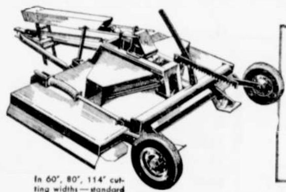
In 60", 80", 114" cutting widths—standard or hydraulic models
