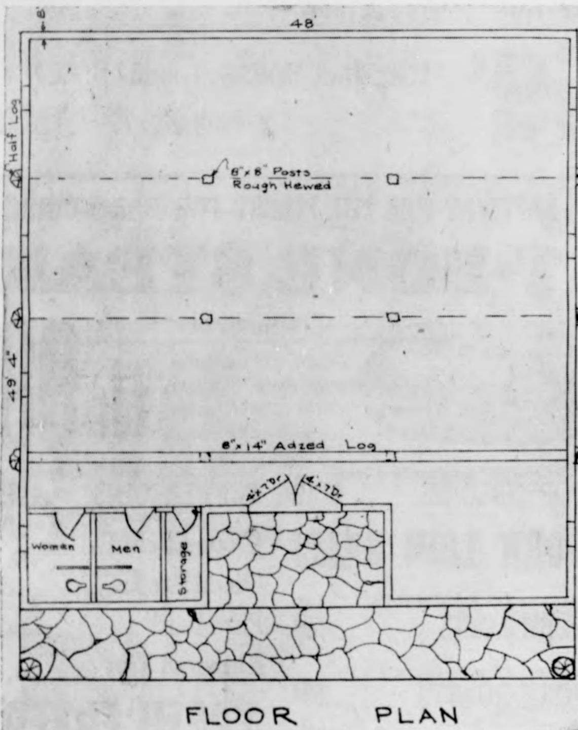
WHEN VOTERS go to the polls in November they will be asked to decide whether to adopt a one-mill levy for raising funds to construct a county historical museum. Artist's drawing above indicates tentative floor plan for structure. Design work was done by Clarence Wagner.
