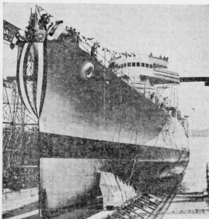
The actual launching of the new United States cruiser Vincennes, at the Fore River plant of the Bethlehem Shipbuilding corporation in Quincy, Mass., is pictured above. The 10,000-ton vessel was christened by Miss Harriet Virginia Kimmell, daughter of the mayor of Vincennes, Ind.
