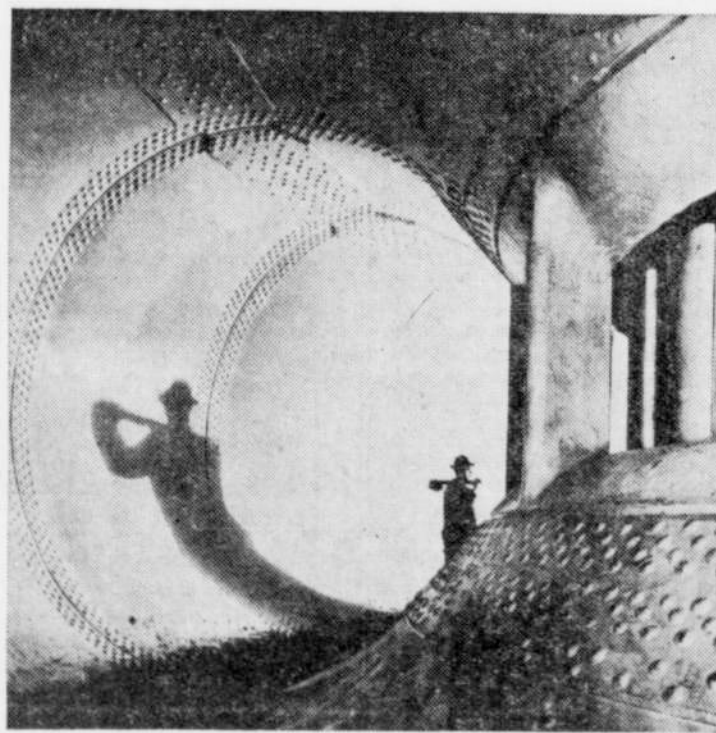
This scroll case at the Norris dam in Tennessee forms the lower end of the penstock or tube which conducts water from Norris lake to the turbines of the power plant. The swirling water will pass through the wicket gates or valves to the right of the workman, and thus into the turbines. There are two of these scrolls at the Norris dam, one for each generator.
