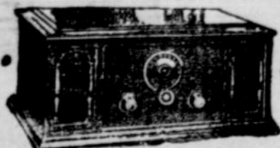
Magnavox 10-5 tube tuned radio frequency, interchangeable receiver unit. Price without tubes or batteries—$110.00
