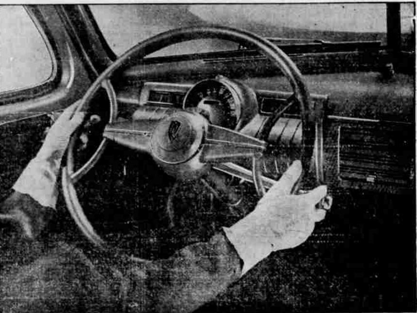
The Oldsmobile automatic safety transmission, obtainable at extra cost on both Six and Eight, is operated by the short lever shown on the steering column. Its position allows three passengers to ride comfortably in front. The clutch is used only to start or stop the car. The new type steering wheel, designed for use with the automatic transmission, affords a clear view of the instrument unit which is directly in front of the driver assuring clear vision.
