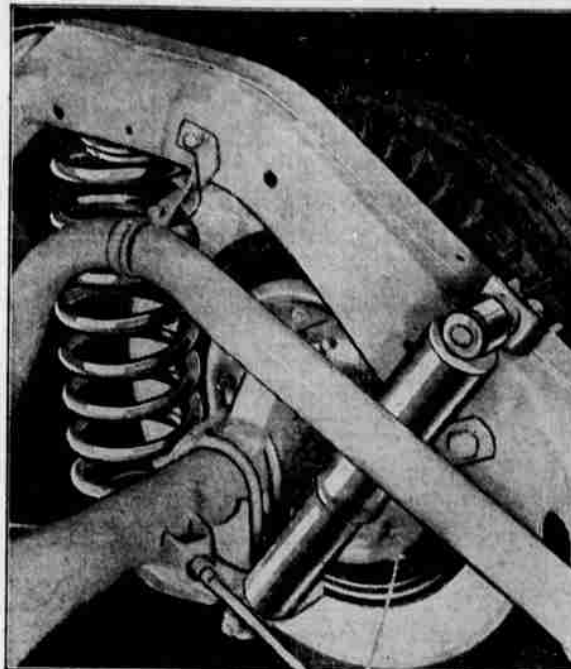
COIL SPRING rear suspension, one of the major automotive developments of the year, has been pioneered by Buick on all four lines of cars for 1938. A feature exclusive to this make, rear coil suspension combines with airplane type shock absorbers to provide greatly improved riding and steering qualities. Photo shows the spring and shock absorber hook-up on the left rear wheel of the 1938 Buick chassis.
