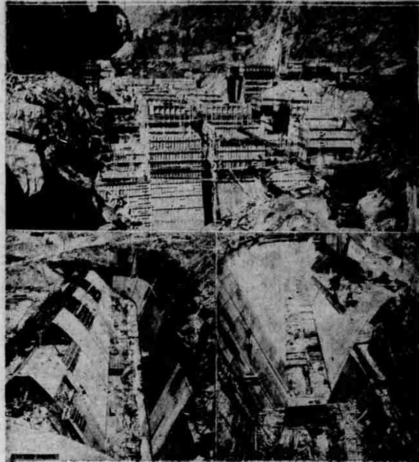
With 2600 men on the job, construction of the Boulder dam goes forward at a rapid pace. Above rough photos depicting progress on the great project show, first, dam to be poured at the canyon, showing the up-and-downstream dimension of the dam base which will fit snugly against the canyon walls at top and left. Below, left, looking upstream at the Nevada spillway. Right, looking upstream at the Arizona spillway.
