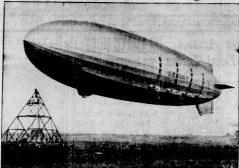
"Up ship!" With this command, the U. S. S. Macon begins her career in the navy. The picture shows the mammoth airship, sister of the lost Akron, at the moment her maiden flight began, just as she cast away from her mooring mast.
