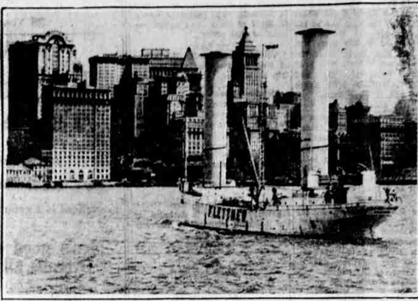
This trim looking yacht-like craft with what seem to be two cumbersome masts and no visible signs of propelling power is attracting attention in New York as it runs about the harbor. It is the Baden Baden , sailless or rotor ship, invention of Anton Flettner, and has just made the trip across the Atlantic under its own power, supplied by the funnel-sails.
