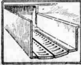
THE WIDE AND SHALLOW FIREBOX Saves Fuel
