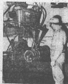
Come in... watch our Twin-Head roller rebuilding machine automatically build up wearing surfaces and flanges with hard steel.
