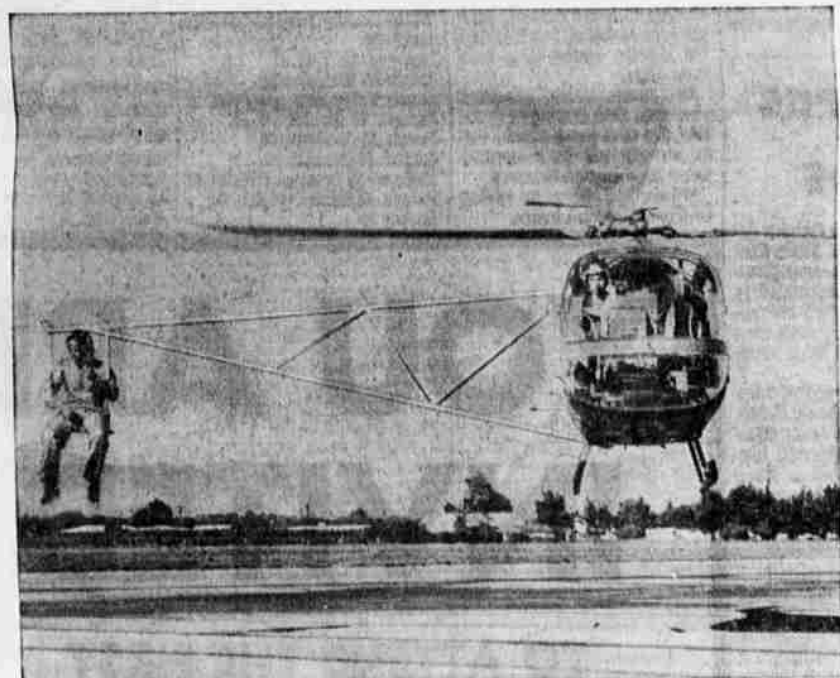
GRAVITY RANGE —This helicopter demonstrates a new, but unique concept in an aircraft's center of gravity. It means varied loads without danger of upset.
