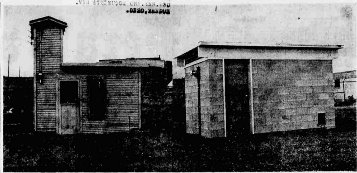
THE OLD AND THE NEW — A new storm water pumping station this week replaced an old one at the foot of Owens Street. The old station (left) was built in 1933, but was found to be inadequate and was torn down to make way for the new facility (right). One pump was transferred to the new station from the old, and two new pumps were installed. Storm drainage water from Mills Addition collects under the station and is pumped into surface ditches. The total project also included the revamping of the storm drain system under Owens and White streets to eliminate flooding. Total cost was $10,000, half of which went for the station. City crews did the work. The station was designed by Robert G. Kyle, city manager.
