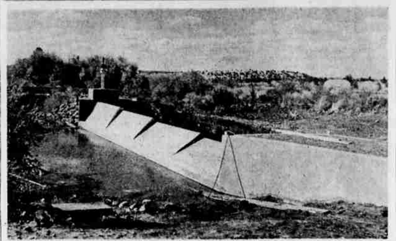
PARKER CREEK DAM — The new Parker Creek Dam and spillway, 10 miles east of Alturas, was recently completed for the Modoc Fish and Wildlife Refuge. The dam features folding sections which can be cranked up or down to regulate the level of the water.
