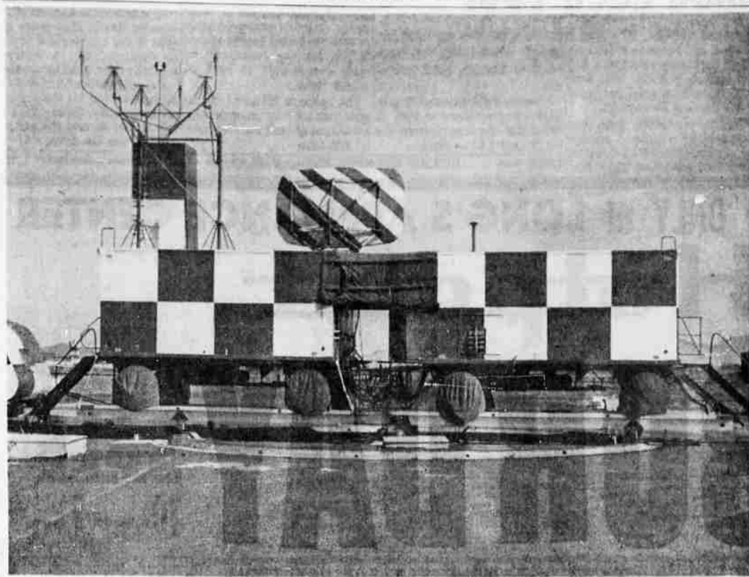
RADAR ON WHEELS —Resting on specially designed track, the GCA van at Kingsley Field is able to rotate 360 degrees so that its precision antennae will always point in the direction of the runway being used for landings.
