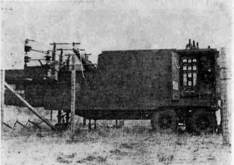
PORTABLE SUBSTATION — This portable substation will take the load off Pacific Power and Light's Pelican City station Tuesday while work is done on the permanent installation. The portable substation is complete in every detail and will handle power for the Pelican City area for two days. The substation is built on a flat-bed trailer and is based in Medford for use in emergencies all over Southern Oregon. It can be in operation in Klamath Falls within six hours of an outage here.
