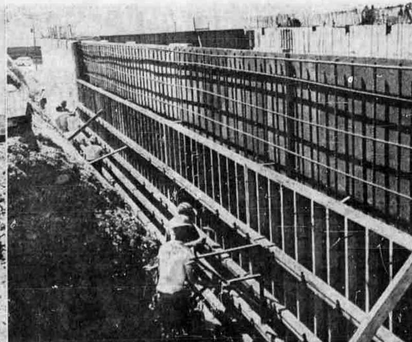
instruction shops, library, radioactive isotopes laboratory building and landscaping of the campus. Center view shows work on the radioactive isotopes laboratory structure. Grading and leveling work on the site of the shops building is shown at left and right. Plans call for occupancy of the campus by fall classes of 1964 at Oregon Tech. At present, huge mounds of earth on the campus obscure portions of the
