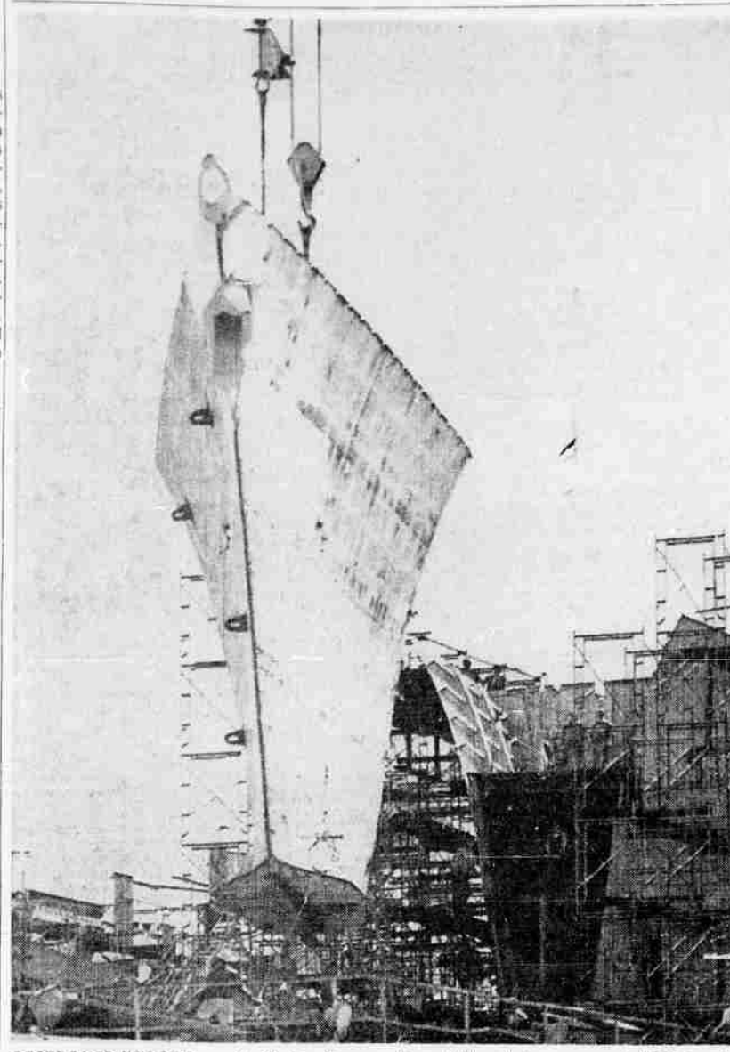
DESTROYER-ESCORT — A 62-ton bow section of the destroyer-escort USS Garcia is lowered into place at the Bethlehem Steel Company's San Francisco yard. Installation of this prefabricated unit means that 98 per cent of the steel for the vessel's hull has now been erected.
