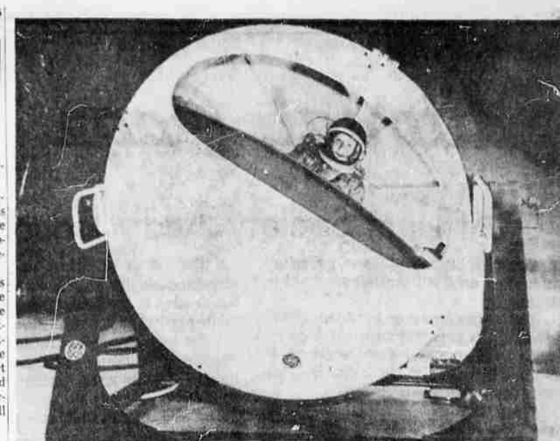
SPACE SHUTTLE — Scientists at Valley Forge, Pa., are working on a space shuttle that would zip back and forth between the earth and orbiting stations carrying supplies for men on the moon. General Electric engineers have built this jet-propelled, land-based "space shuttle" that simulates a landing on an orbiting vehicle.
