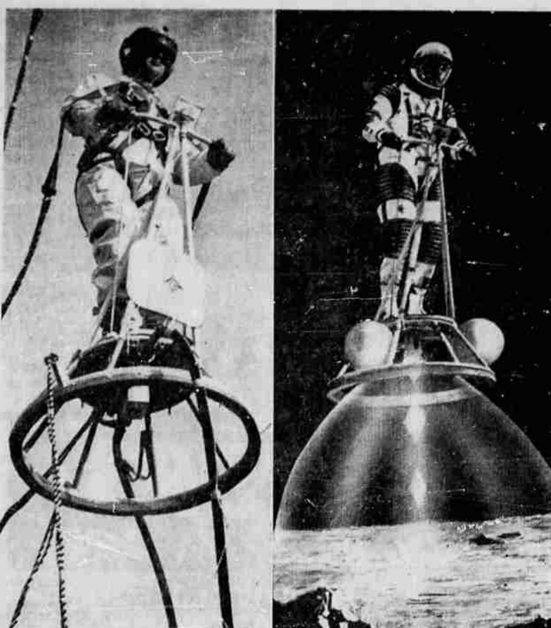
SPACE SCOOTER — Here is a flying space scooter that can hover, rotate, accelerate forward, backward or horizontally and descend for a soft touchdown. The scooter is being tested at North American Aviation in Los Angeles. —UPI Telephoto
