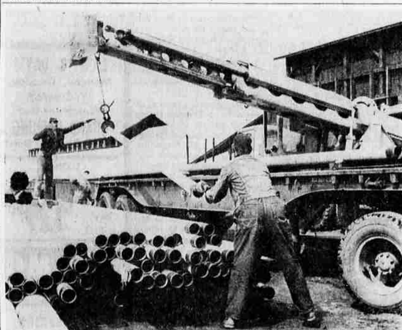
PIPE LAYER —This machine will load, unload, and assist in pipe laying. California-Pacific Utilities Company has let the contract to Bud Stump, Klamath Falls, to lay about five miles of pipe for natural gas at an estimated cost of $130,000. Here Lee Winter, left, and J. F. Rusher are busy loading up pipe which is being laid out adjacent to Kit Carson Way and on into Pelican City.
