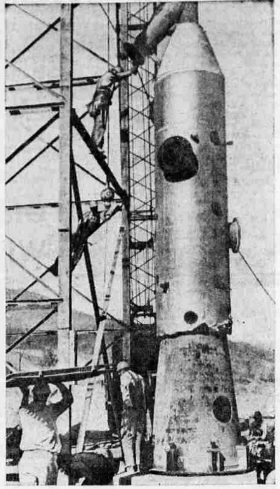
KEEP COOL —No, it's not a missile, but a cooling unit of the concrete batch plant now being built at the site of the Oroville (Calif.) Dam, a key unit of the State Water Plan. The dam will stand 735 feet high when completed.
