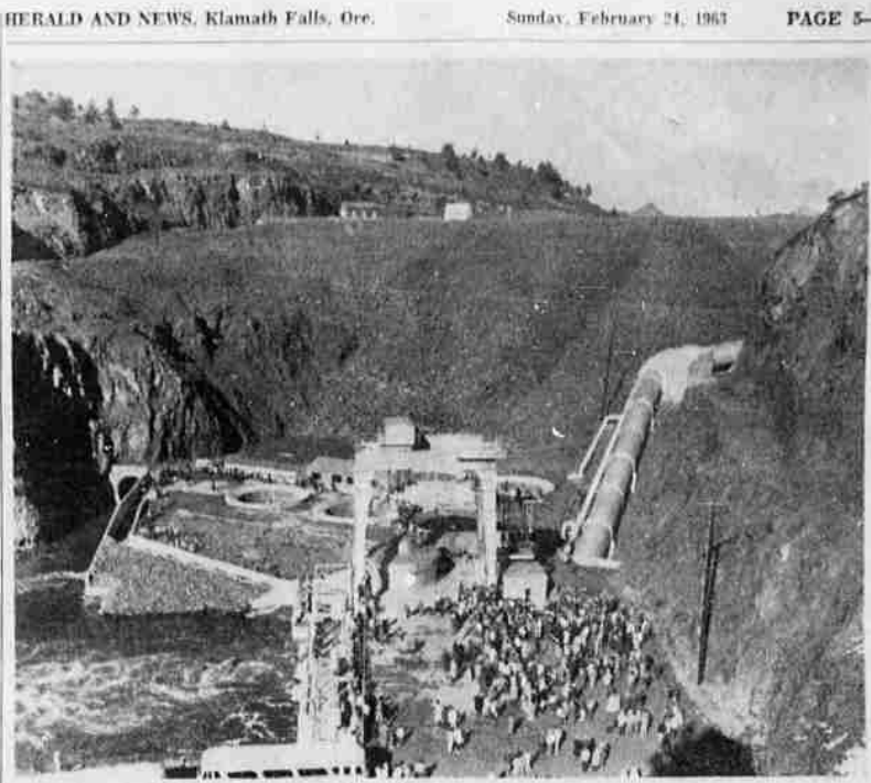
BIG JOB COMPLETED — One of Pacific Power and Light Company's largest construction projects completed last year was the Iron Gate Dam on the Klamath River. Major purpose of the $7,500,000 dam was to regulate flow of the river downstream. This view shows the project on the day it was officially dedicated on Feb. 1, 1962.
