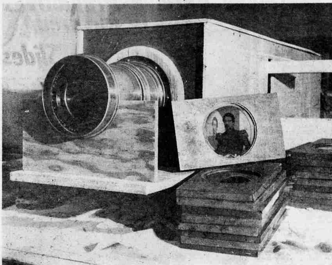
A HOME-MADE slide projector is used to show the heavy wood-mounted slides. Main lens on the projector is from an old portrait camera.
