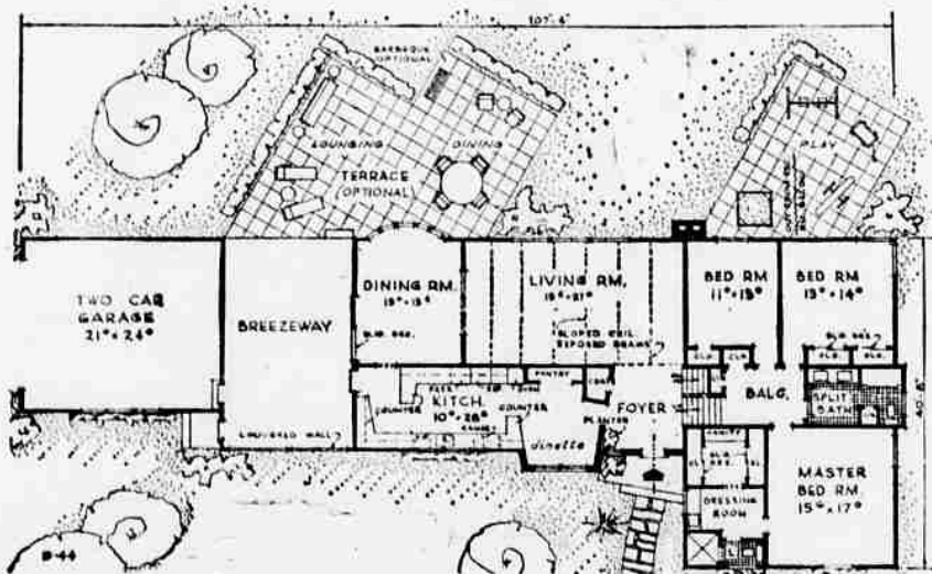
FLOOR PLAN: An angled wall across one side of foyer lends distinction to this three bedroom split level. Note the long kitchen with its splendidly spacious counters.
