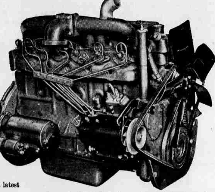
International D-301 Engine gives you low-cost diesel performance for the short haul. Naturally aspirated 301 cu. in. engine delivers 110 hp. at 3,000 rpm. Weighs only 902 lbs. or 8.2 lbs. per horsepower. High torque output at low speed, low fuel consumption and long life between overhauls have been proven in actual truck use. Direct electric starting and a simplified fuel system are other advantages. Heavy-duty construction features include fully-hardened crankshaft and reinforced crankcase.
