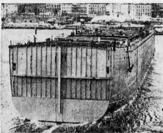
HALF A SHIP —A strange vessel, without bow or stern, was seen after launching at a shipyard in Hamburg, Germany. The nameless 510-foot ship will be towed across the Atlantic and grafted onto the former 17,000-ton tanker "Chiwawa." The hybrid ship will be used as an iron ore carrier.
