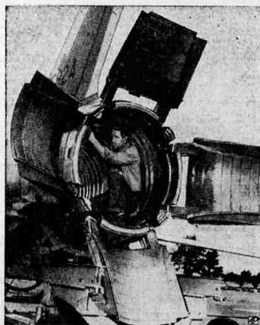
PUSH 'N' HOLD — Workman adjusts the speed brake assembly at rear of F-105 fighter-bomber. Opened, they act as brake; closed, they add thrust to jet engine.
