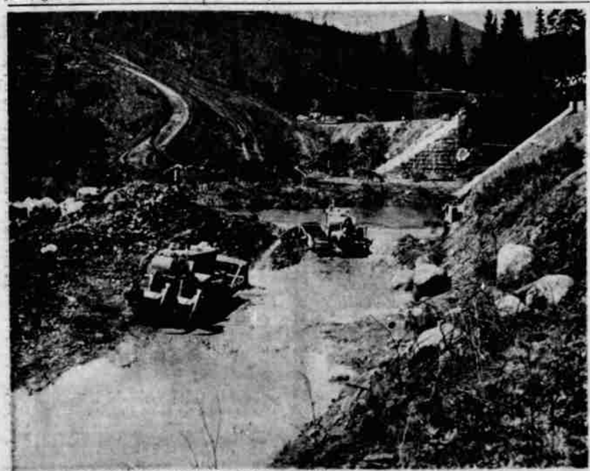
A BOW IN THE SACRAMENTO RIVER was eliminated last week when the Morrison-Knudsen Construction Company changed the channel of the river near Castle Crags, four miles south of Dunsmuir. This change will eliminate high water dangers to the Southern Pacific railroad tracks and the new freeway during the heavy spring runoffs. The railroad company and the state highway department worked jointly on the relocation of the channel with the S.P. Company arranging to move the channel and do the necessary grading for the railroad roadbed and the river channel.
