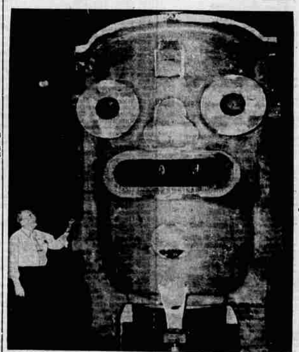
MAN AND THE IRON MASK —Warrior-like mask is part of a giant steam turbine-generator unit. The unit is 18 feet high, weighs 15 tons. Markings on the face are guides for machining and drilling operations. "Mouth" admits high-pressure steam from boiler into turbine. Steam is then returned to boiler for reheating and then readmitted to turbine through the "eyes." It was made for use in Puerto Rico by GE in Lynn, Mass.
