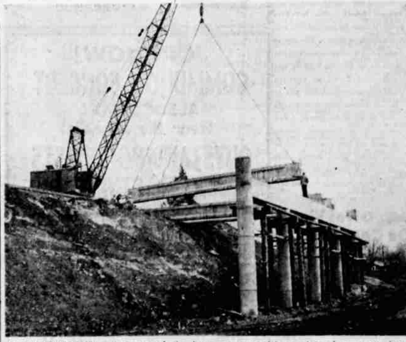
A GIANT CRANE swings one of the huge pre-stressed beams into place as construction moves forward on the Nevada Street interchange of the West Side Bypass. The overpass at this point will be 166 feet long and will provide a 63 foot clear roadway. The Tom Lillebo Construction Company of Reedsport is utilizing pre-stressed concrete beams on concrete column bents. This same company has the contract for the bridges across the A Canal and over California Street. Completion of the route, including structures and paving is expected in late 1959 or early 1960.
