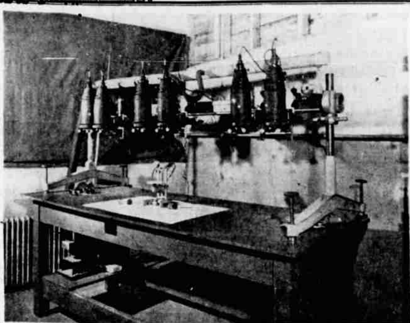
NEW instructional equipment for use of students in photogrammetry classes at Oregon Tech is shown. The Bausch & Lomb Multiplex mapping machine will be used by students in highway technology and surveying technology to practice cartography and put into use their classroom theory. Machine operates on the same stereoscopic principle as 3-D movies. Each pair of projectors has red and green filters and the operator wears spectacles with red and green color for each eye. By manipulating a floating dot of light on the tracing table, accurate vertical and horizontal distances can be traced on a map manuscript. This method, with some variation also lends itself to reconnaissance and planning of highways and hydroelectric systems.
