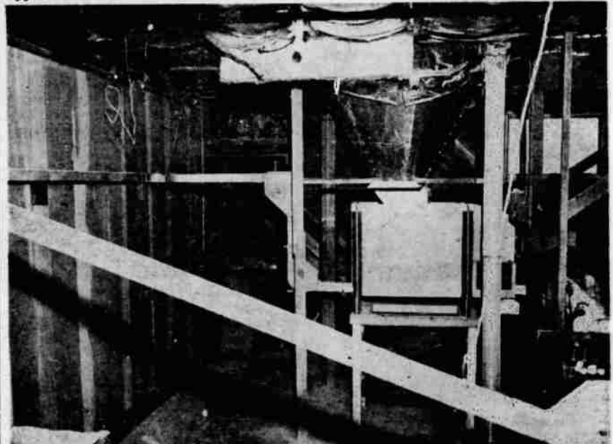
FEED UNIT for one of the two automatic feeding systems in the new cage house at Gooding Poultry Farm shows the hopper arrangement which drops the proper amount of dry feed onto the chain feeder for distribution throughout the building. Each system can feed more than 3500 birds at a feeding.
