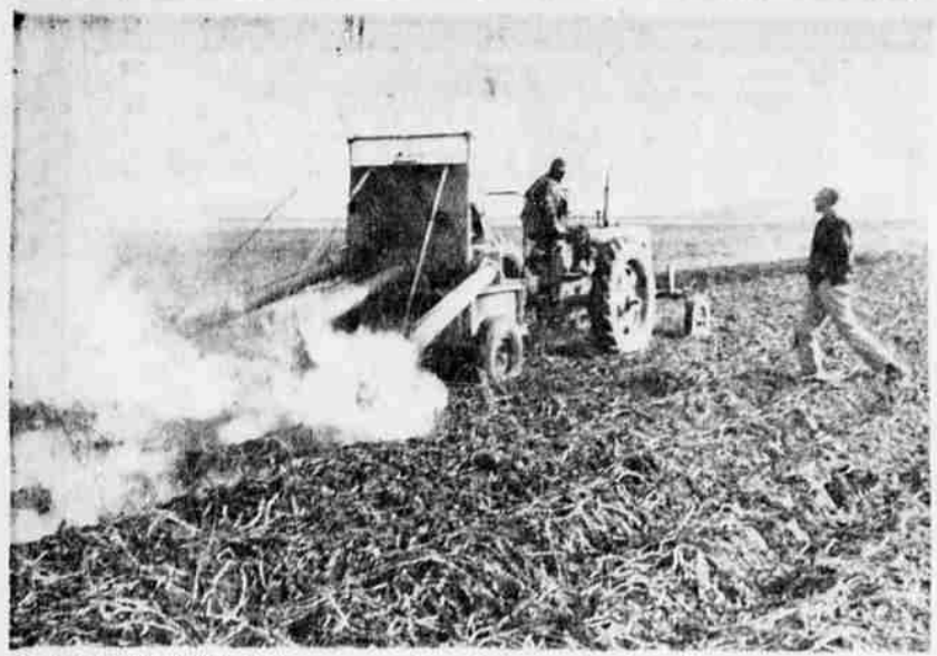
A CLOSE UP VIEW of the new experimental burner is shown here as it works in a field. Each pass covers a four-row width, and can cover 40 to 60 acres per day at a fuel cost of about $5 per acre. It operates at a speed of about five miles per hour.
