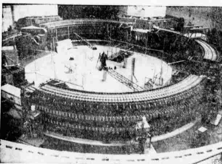
FRENCH ATOM SMASHER — This is a general view of the "Soleil" France's new synchro-cyclotron which has gone into operation in Saclay near Paris. A heavy protective concrete wall surrounds machine, believed largest of its type in world.
