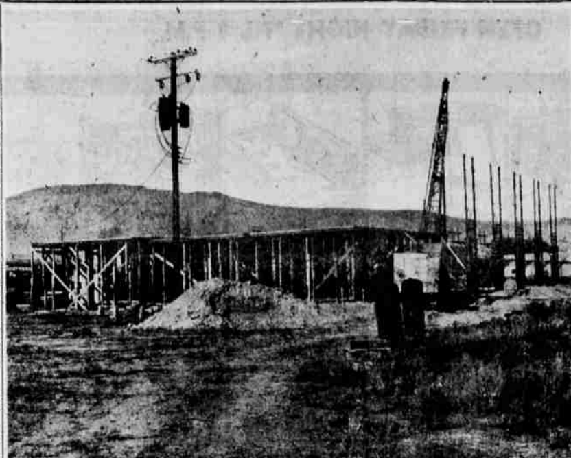
COUNTY ROAD MAINTENANCE shops will move into this $131,000 building scheduled for completion about December 1. Included will be a 20-ton bridge crane, believed to be the only such crane in any highway department west of the Rockies. Howard and Morrison are contractors for the building, on Washburn Way, which will replace the present shop on the county fairgrounds.
