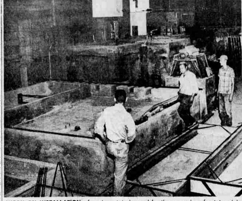
WORK ON INSTALLATION of equipment to be used for the processing of potatoes into starch is moving on schedule and the plant will be ready to open in time for the fall potato harvest. These concrete tanks are for washing starch during the process of converting potatoes to the by-product. The plant, to be located at Hatfield, California, is the Western Starch Company. Marvin J. Aslett, St. Anthony, Idaho, is president. Left to right in the picture are Garth Powell, recently of Moses Lake, Washington, plant manager; Ben Gorton and LeRoy Moulds, assisting with setting up the machinery. The dry starch produced here will be used in the production of glass paper.
