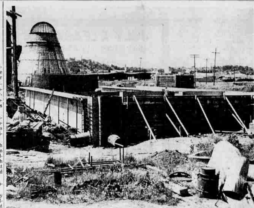
CONSIDERABLE PROGRESS was being shown in this picture of construction of the new primary sewage treatment plant. The plant is being built by the H. G. Carl Construction Company of Salem at a cost of $238,386.29 on a site on the shore of Lake Bosworth midway between Klamath Avenue and the Great Northern Railroad tracks. They were awarded the bid by the city council on January 13. No date for completion has yet been set, but indications are that it will be finished by early fall. The L. F. Henshaw Company of Eugene was awarded the bid last night to build the secondary treatment plant which will be adjacent to this plant. The Henshaw bid was in the amount of $136,413. Completion of these two plants will give the city of Klamath Falls a complete conventional sewage treatment plant.
