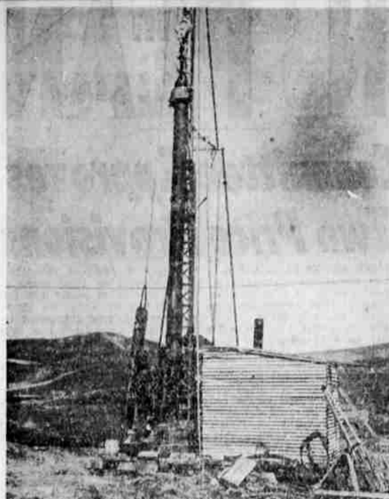
A HOT WATER FLOW has been tapped by this well drilling machinery to be used for heating the new junior high school which will be located to the right of the highway to Oregon Technical Institute. Some leveling for the proposed building was done last fall. Drilling operations were done by E. E. Storey, 4237 Summers Lane, back to camera. Assisting him has been Joe McLane, general delivery, this city. The well, down 463 feet, is being cased. Temperature of the water is 209 degrees.
