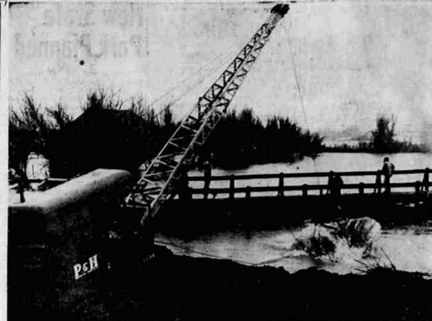
A DRAGLINE was used to protect railroad bridges at Alturas during the flood Sunday which inundated a square mile of the Northern California community. Debris piled against the span shown above and the force of the current threatened to sweep the structure away. — Photo by Don Kettler
