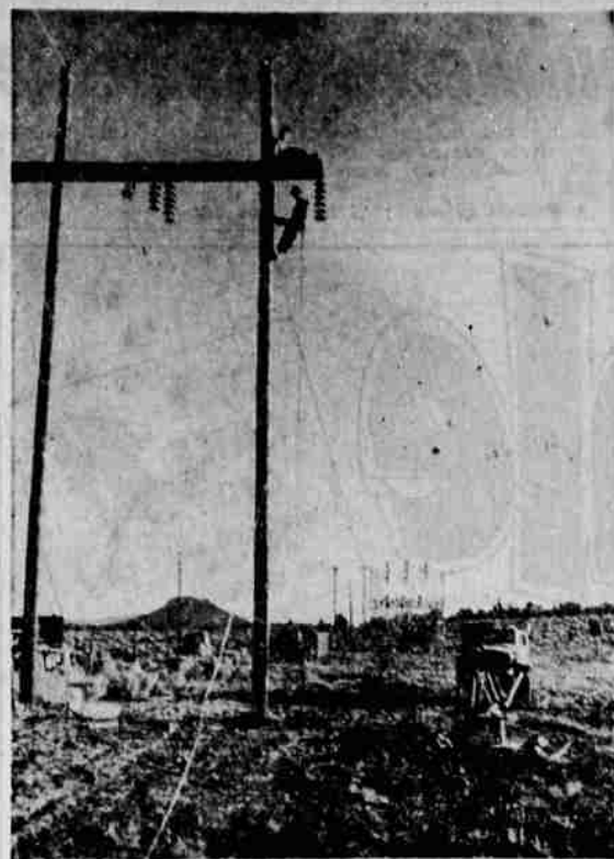
END OF THE LINE for the 150-mile electrical distributive system which is bringing rural electrification from Midstate Electric Cooperative at LaPine to the Fort Rock-Silver Lake area was this double-pole, H-type dead end assembly set up as the last unit at the Silver Lake substation. Work was done by Carlson Construction Company. Workmen are shown attaching the conductor cables to pole number 537. The line will be energized at a public celebration Friday. —Photo by Parks
