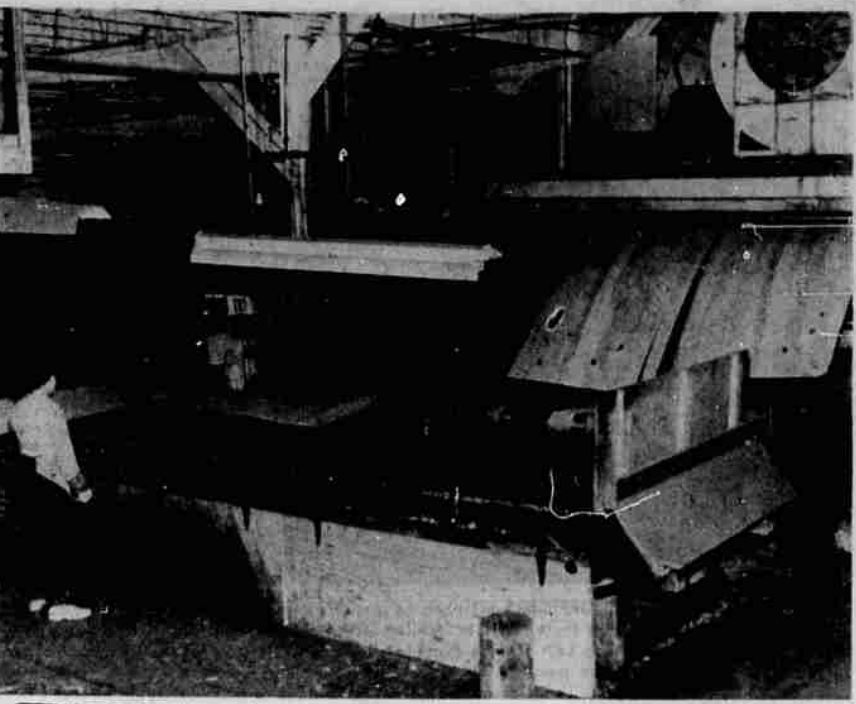
DRIED VENEER GRADER Thelma Claunch marks the various grading symbols on the dried sheets as they come out of the drying machine at the Kalpine Plywood Plant. The various grades of plywood are stacked in piles by other workers to the left of the picture as they move on the belts.
