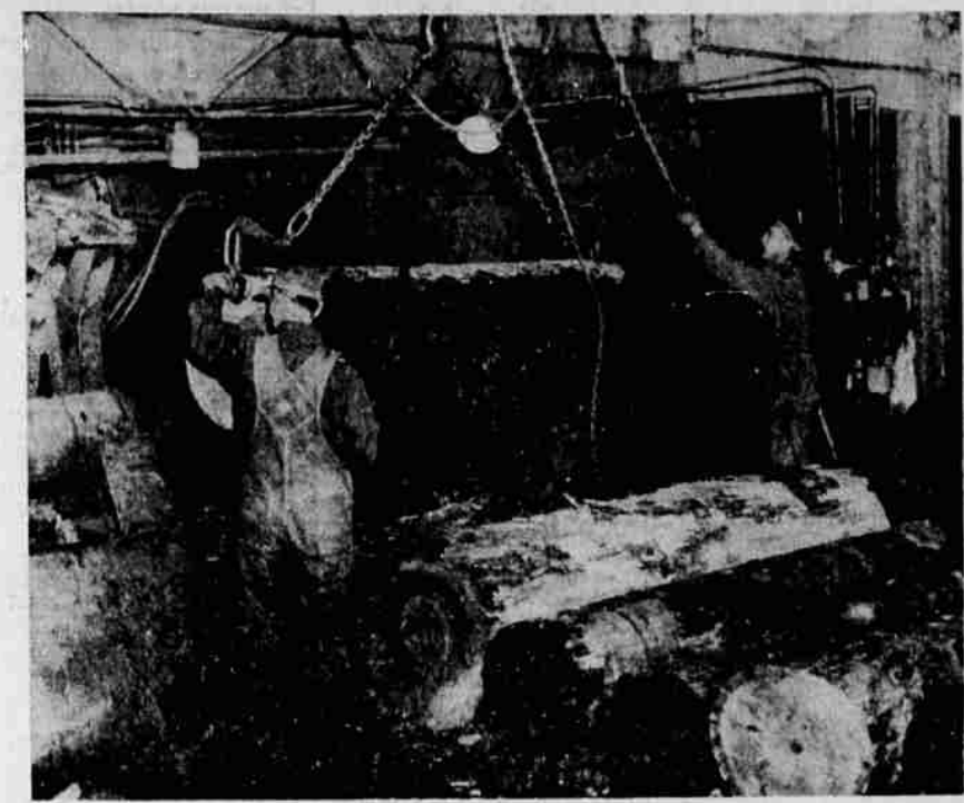
DEBARKING FIR PEELER LOGS at the Karpine Plywood plant are Arkus Bray, right, operator, and Eugene Mayfield. The machine, designed and built by Guy Hand, plant master mechanic, clamps the logs and debarks them as they are turning.
