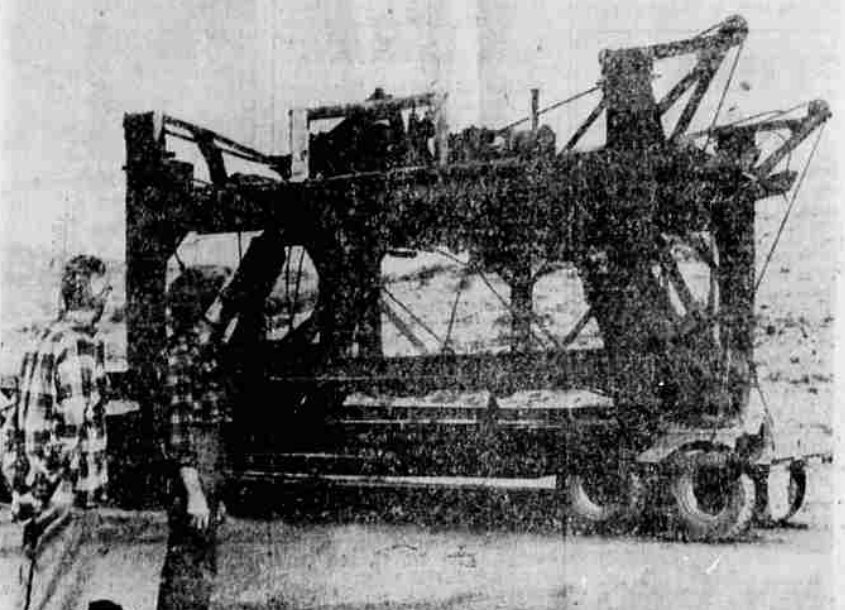
THE FIRST MCGIFFERT LOADER used by the Weed Lumber Company is shown on its way to the Collier Logging Museum on U. S. 97 north of Crater Lake junction (above) as W. R. Robertson (left), weighmaster, and E. F. Anderson look on. In the side photo, the loader is shown on Weed Lumber Company operations in 1929, when it was new. The loader straddled a railway track, and log cars were pushed under it to loading position, where the logs were swung aboard. The six-man crew could load about 100,000 feet a day at from 5,000-7,000 feet per car. The loader could lower wheels from its bed to the track, and then was capable of moving on the track under its own power, or being coupled to a train for a longer haul. Modern versions of this loader will load either rail cars or logging trucks. This loader was sold to Weyerhaeuser Timber Company in 1929. —Old time photo from Lou Parsons' collection loaned by A. D. Collier.
