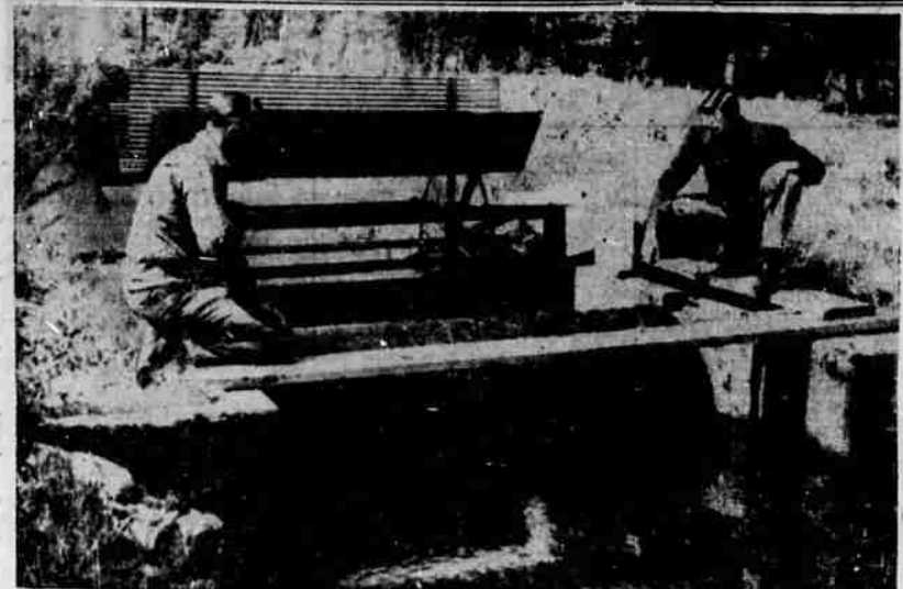
LITTLE PADDLE WHEELS save the lives of many Oregon fish by keeping them out of irrigation ditches. This paddle wheel creates a current which turns a rotary screen, over which the fish can't pass. This one is on the Rogue River near Gold Hill. These devices were invented by the Oregon Game Commission. Some 250 are being installed in the John Day watershed, and 200 others are being used on streams over the state.
